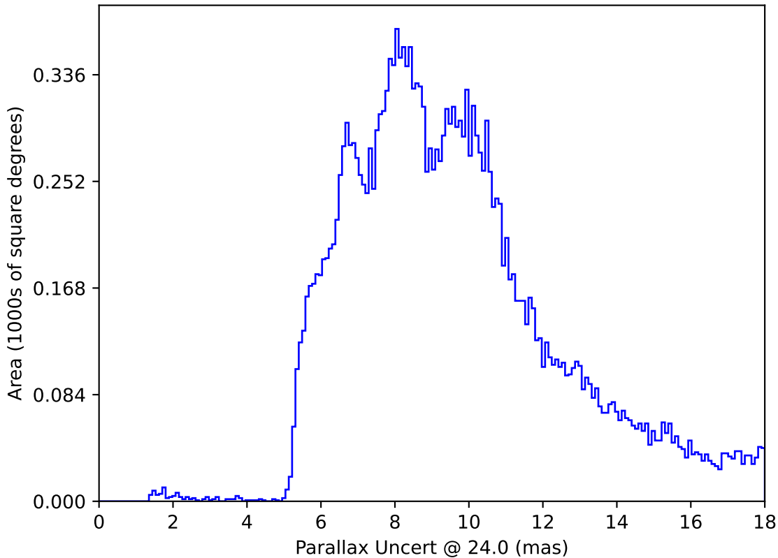
too_elab_r32_d2_ugrizy_v3.4_10yrs All sky: Parallax Uncert @ 24.0
