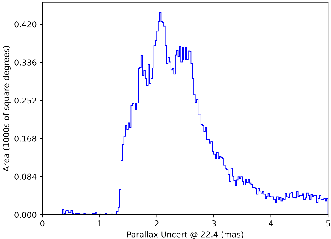
too_elab_r32_d2_ugrizy_v3.4_10yrs All sky: Parallax Uncert @ 22.4
