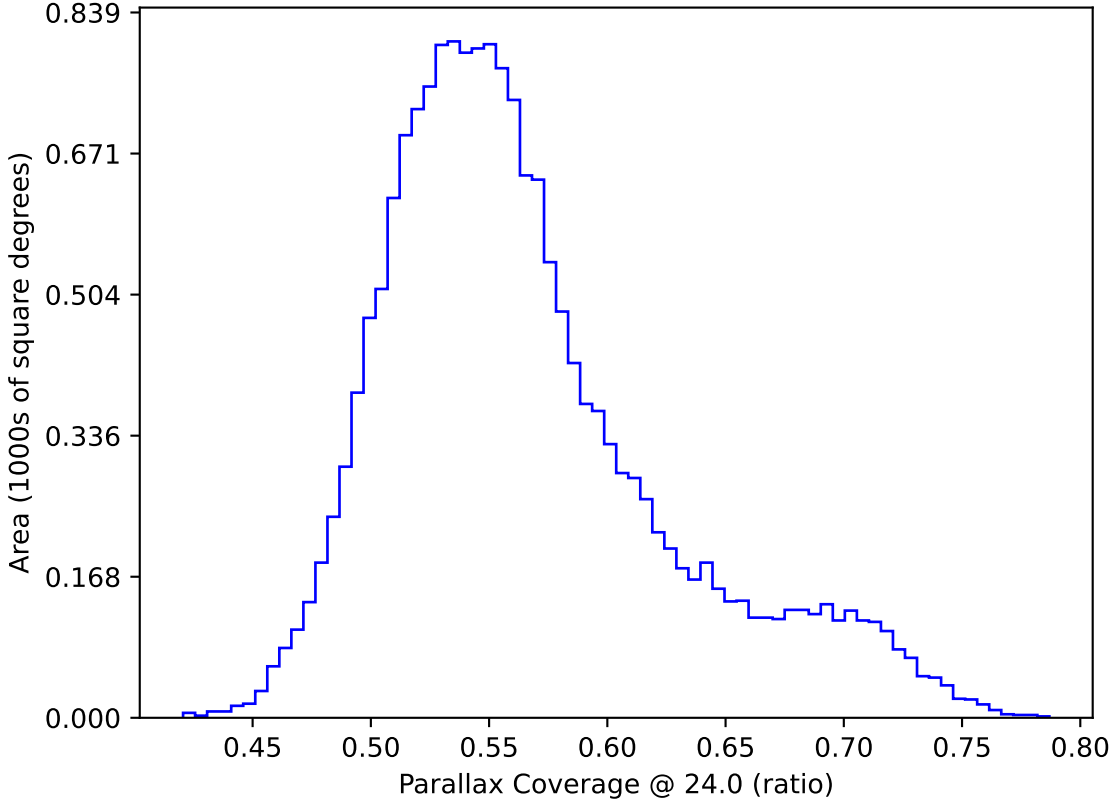
too_elab_r32_d2_ugrizy_v3.4_10yrs WFD: Parallax Coverage @ 24.0
