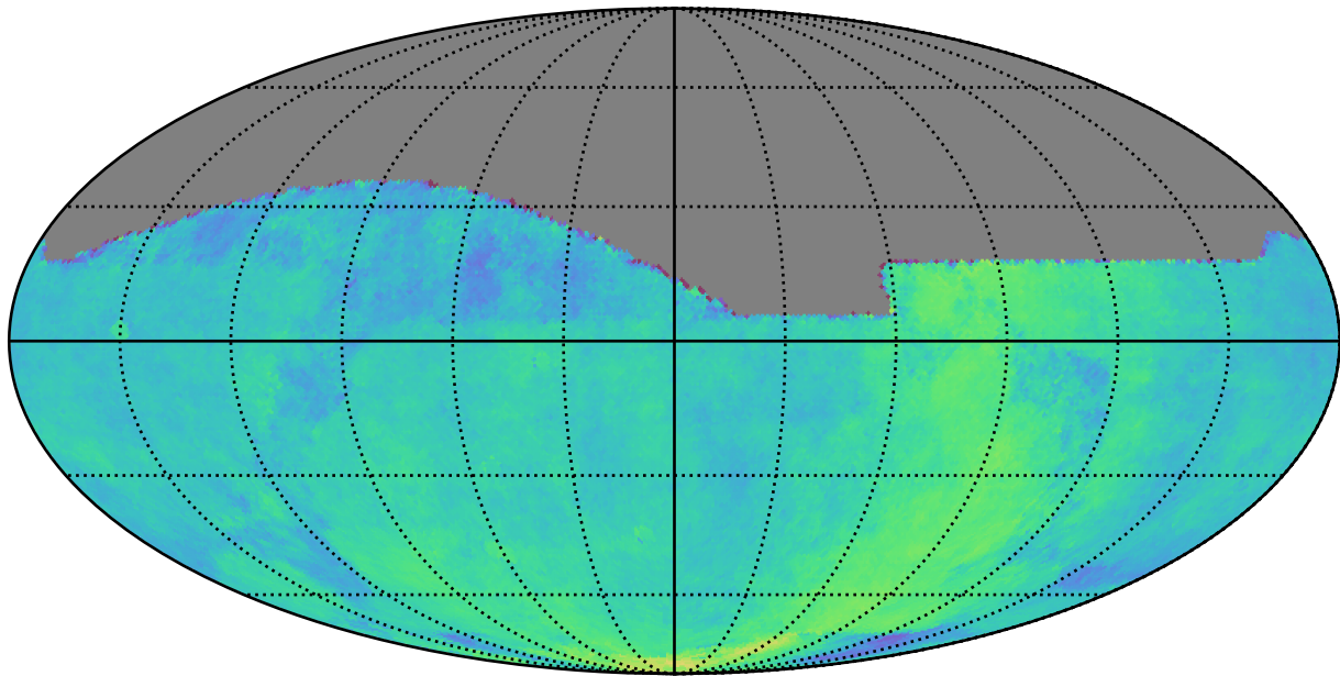
too_elab_r32_d2_ugrizy_v3.4_10yrs All sky: Parallax Coverage @ 24.0
