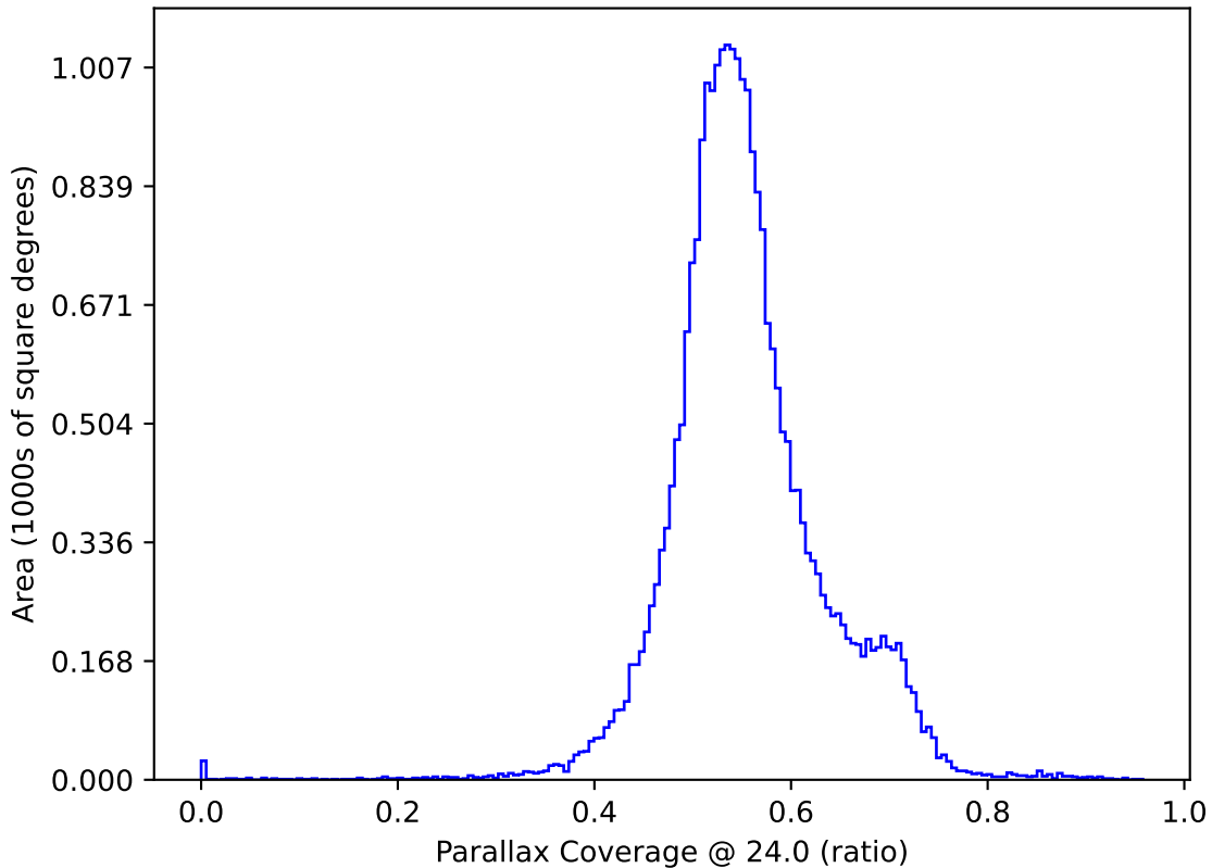
too_elab_r32_d2_ugrizy_v3.4_10yrs All sky: Parallax Coverage @ 24.0
