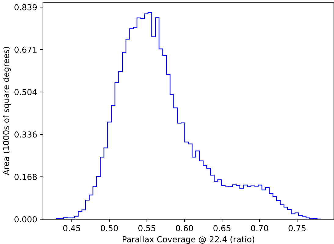
too_elab_r32_d2_ugrizy_v3.4_10yrs WFD: Parallax Coverage @ 22.4
