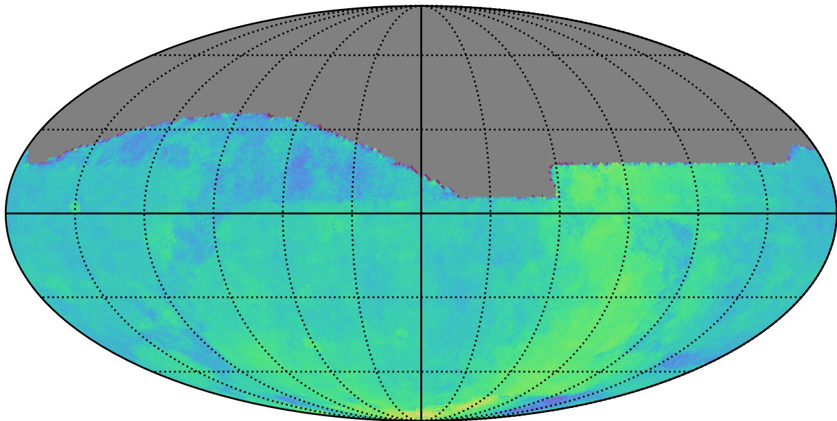
too_elab_r32_d2_ugrizy_v3.4_10yrs All sky: Parallax Coverage @ 22.4
