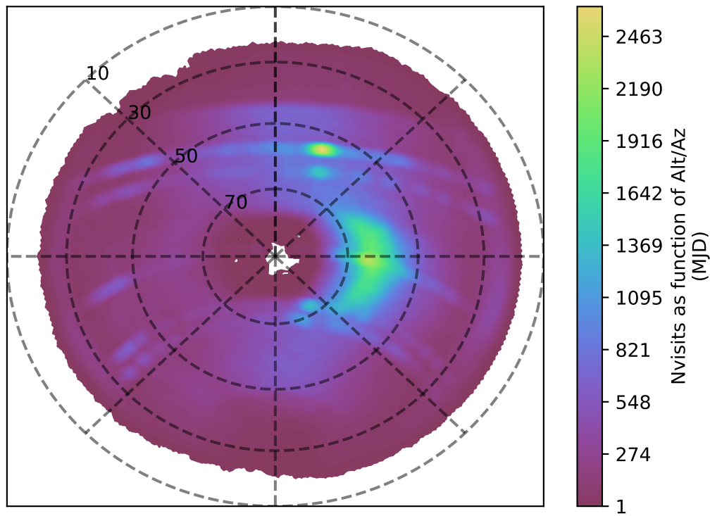
too_elab_r32_d2_ugrizy_v3.4_10yrs z band: Nvisits as function of Alt/Az
