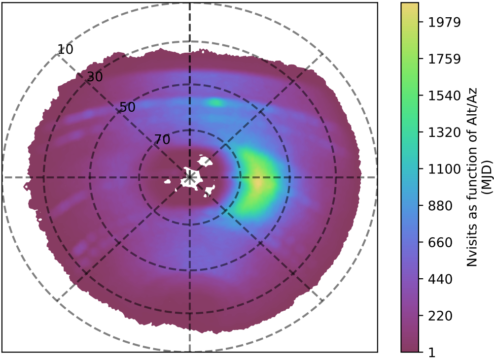
too_elab_r32_d2_ugrizy_v3.4_10yrs y band: Nvisits as function of Alt/Az
