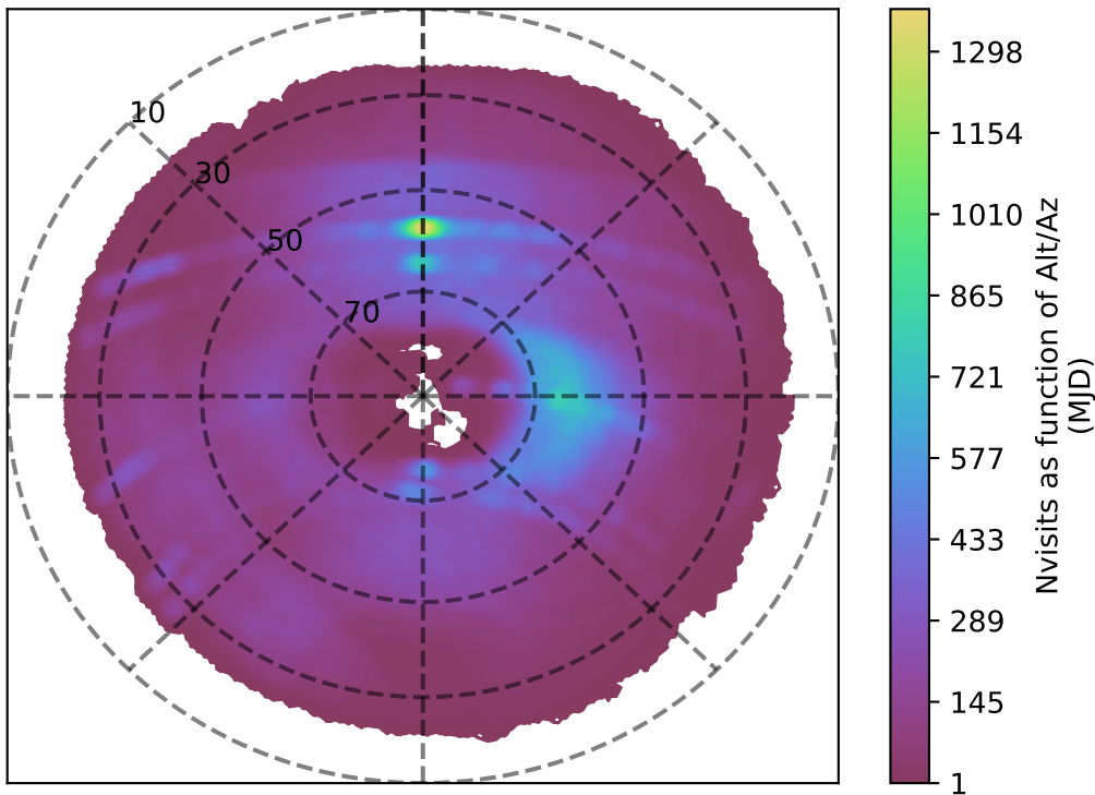
too_elab_r32_d2_ugrizy_v3.4_10yrs g band: Nvisits as function of Alt/Az
