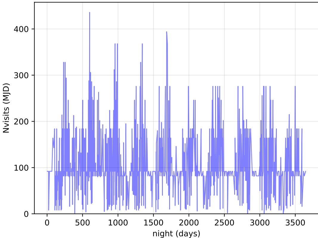
too_elab_r32_d2_ugrizy_v3.4_10yrs DDF: Nvisits
