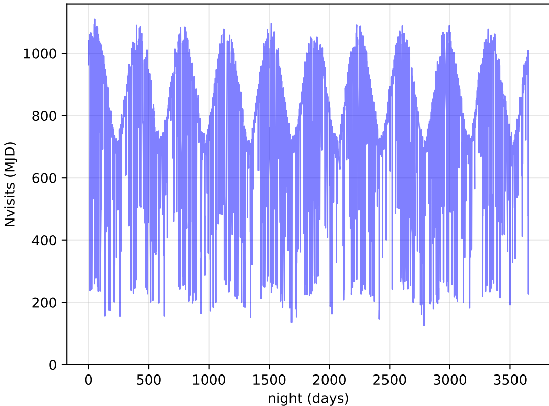
too_elab_r32_d2_ugrizy_v3.4_10yrs All visits: Nvisits
