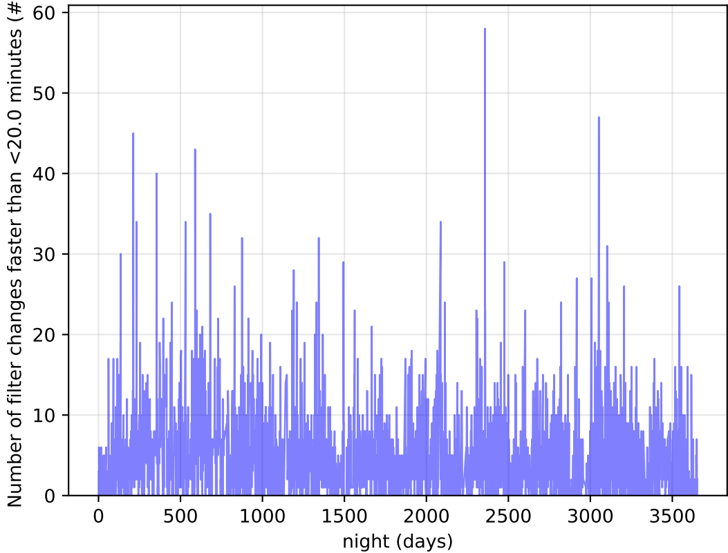
too_elab_r32_d2_ugrizy_v3.4_10yrs Per Night: Number of filter changes faster than <20.0 minutes
