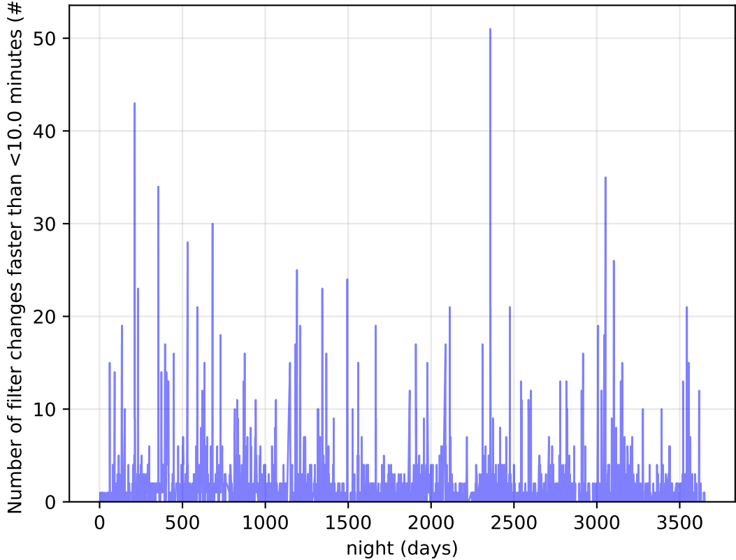
too_elab_r32_d2_ugrizy_v3.4_10yrs Per Night: Number of filter changes faster than <10.0 minutes
