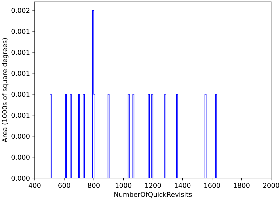
too_elab_r32_d2_ugrizy_v3.4_10yrs WFD: NumberOfQuickRevisits
