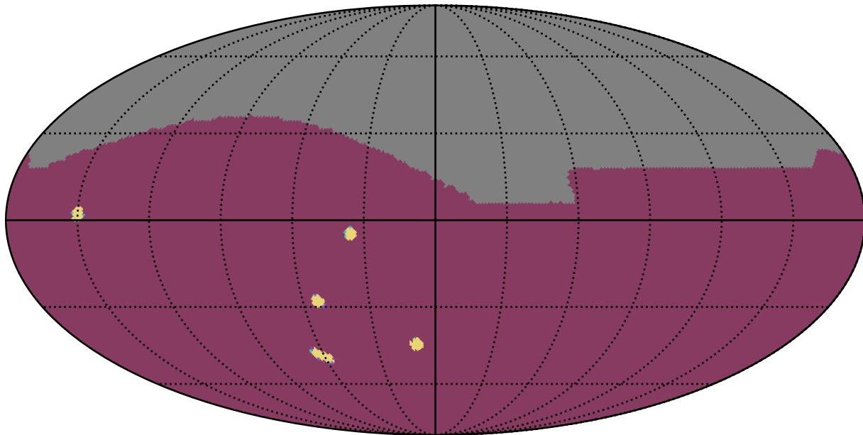
too_elab_r32_d2_ugrizy_v3.4_10yrs All sky: NumberOfQuickRevisits
