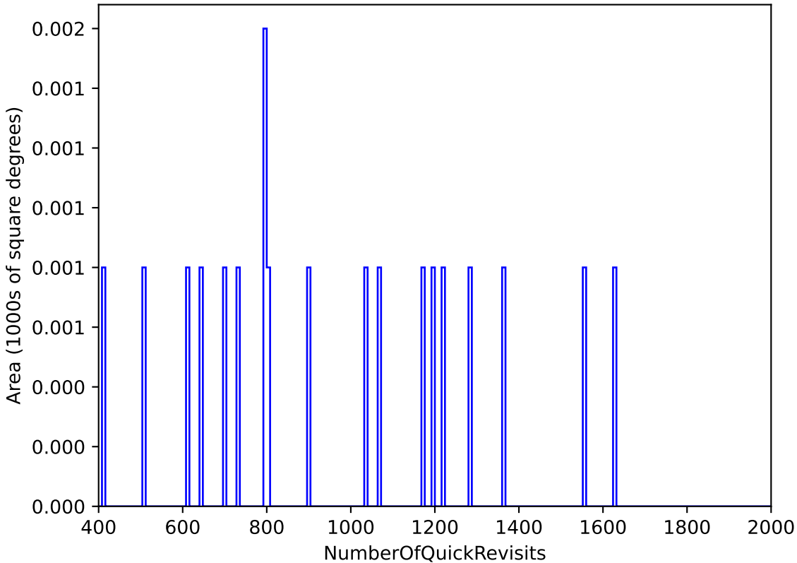
too_elab_r32_d2_ugrizy_v3.4_10yrs All sky: NumberOfQuickRevisits
