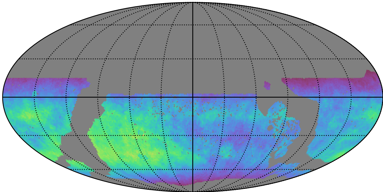
too_elab_r32_d2_ugrizy_v3.4_10yrs WFD z band: Normalized Teff
