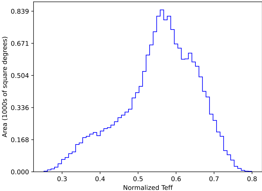
too_elab_r32_d2_ugrizy_v3.4_10yrs WFD y band: Normalized Teff
