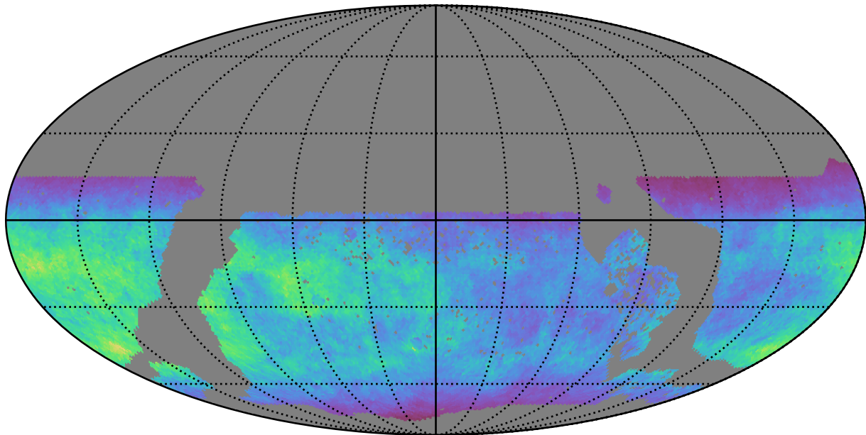
too_elab_r32_d2_ugrizy_v3.4_10yrs WFD u band: Normalized Teff
