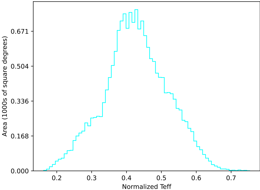
too_elab_r32_d2_ugrizy_v3.4_10yrs WFD u band: Normalized Teff
