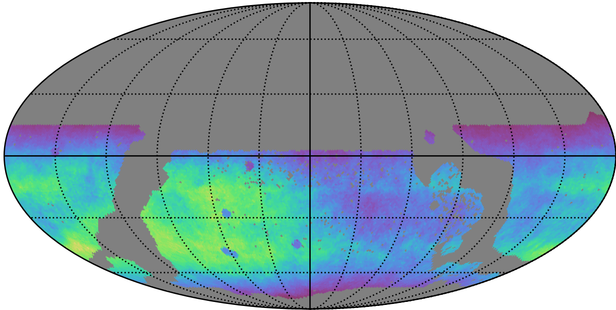
too_elab_r32_d2_ugrizy_v3.4_10yrs WFD r band: Normalized Teff
