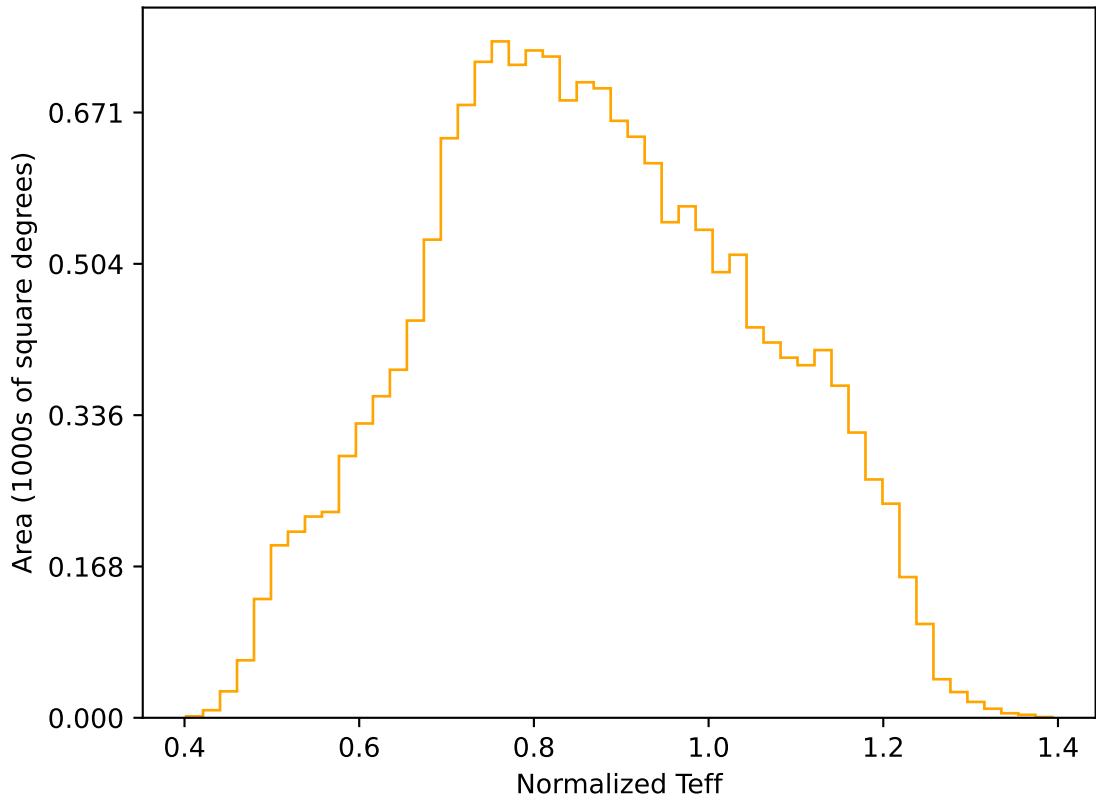
too_elab_r32_d2_ugrizy_v3.4_10yrs WFD r band: Normalized Teff
