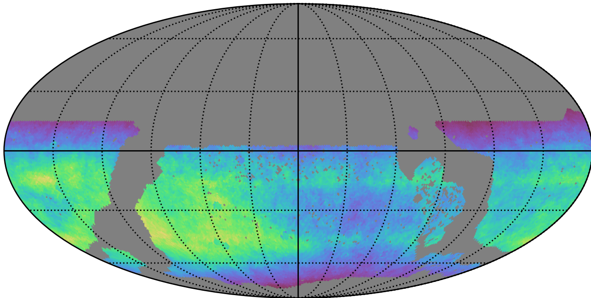
too_elab_r32_d2_ugrizy_v3.4_10yrs WFD i band: Normalized Teff
