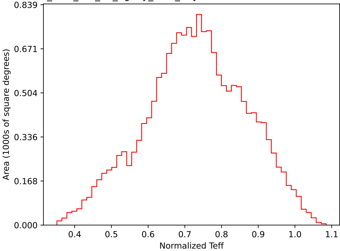
too_elab_r32_d2_ugrizy_v3.4_10yrs WFD i band: Normalized Teff
