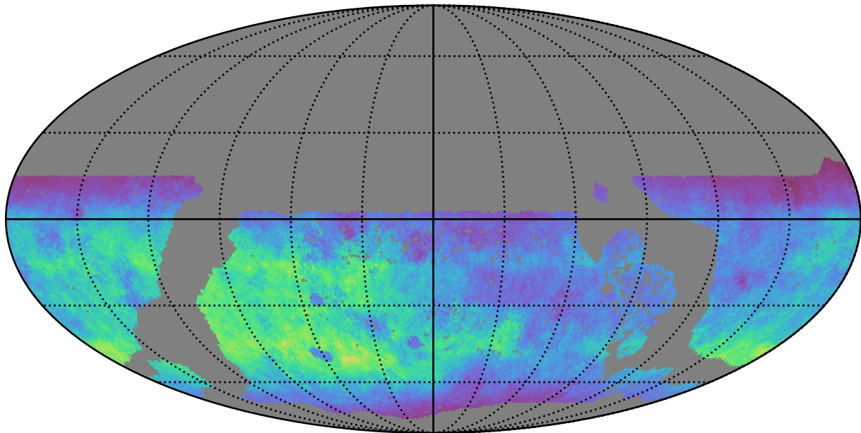
too_elab_r32_d2_ugrizy_v3.4_10yrs WFD g band: Normalized Teff
