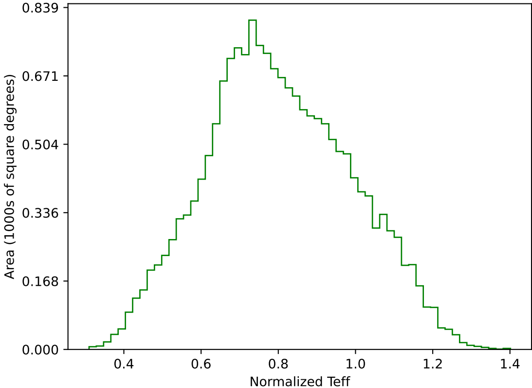
too_elab_r32_d2_ugrizy_v3.4_10yrs WFD g band: Normalized Teff
