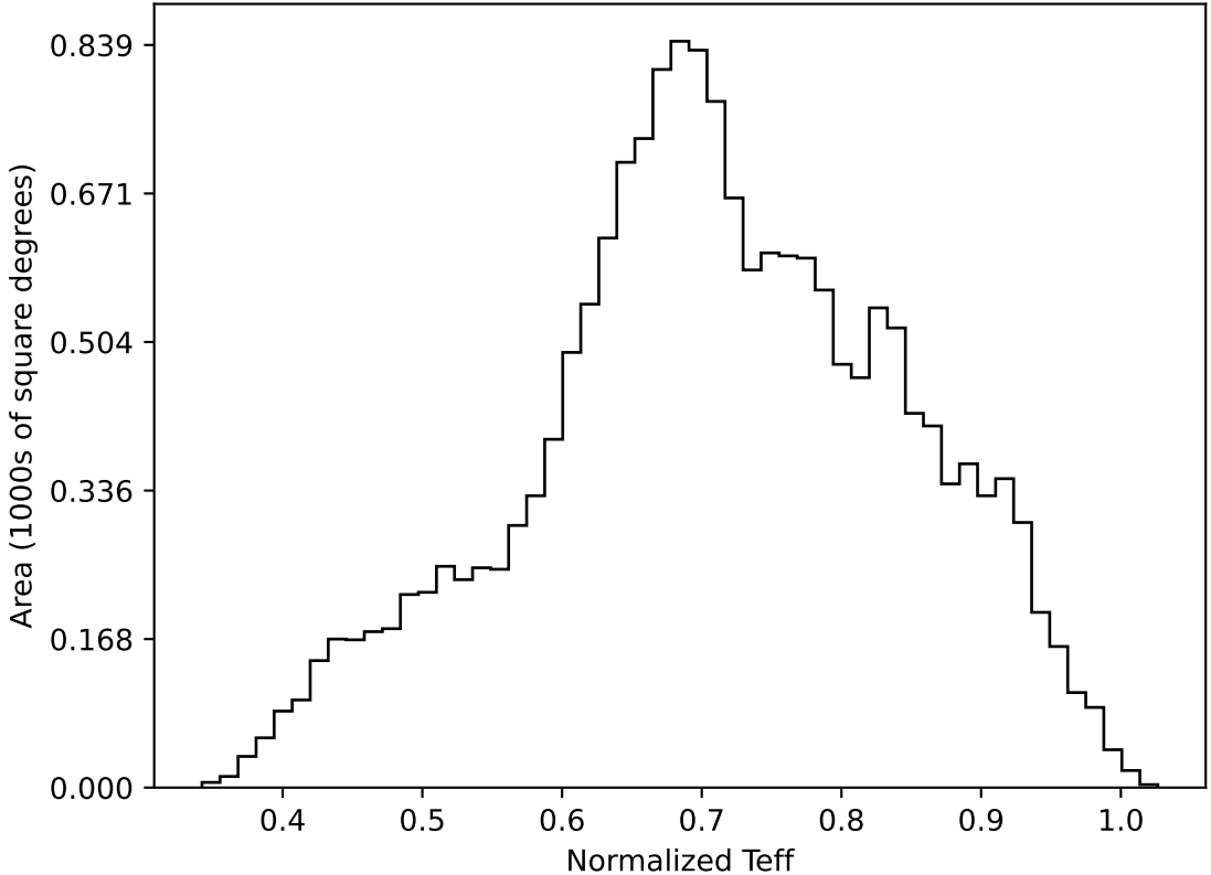
too_elab_r32_d2_ugrizy_v3.4_10yrs WFD all bands: Normalized Teff
