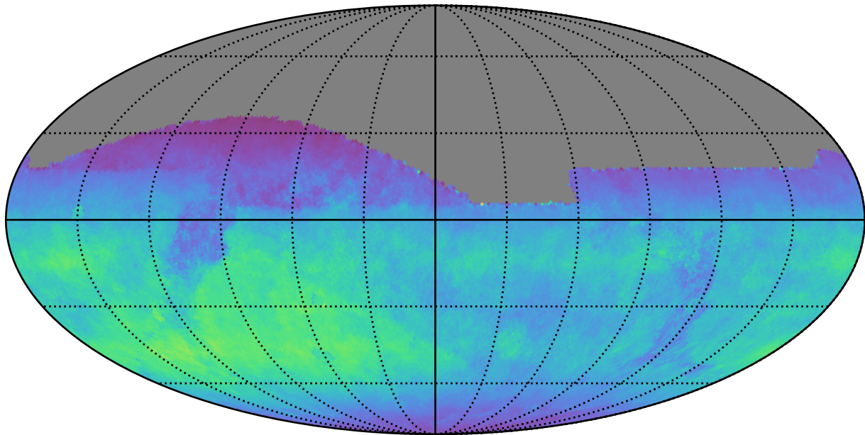
too_elab_r32_d2_ugrizy_v3.4_10yrs All sky z band: Normalized Teff
