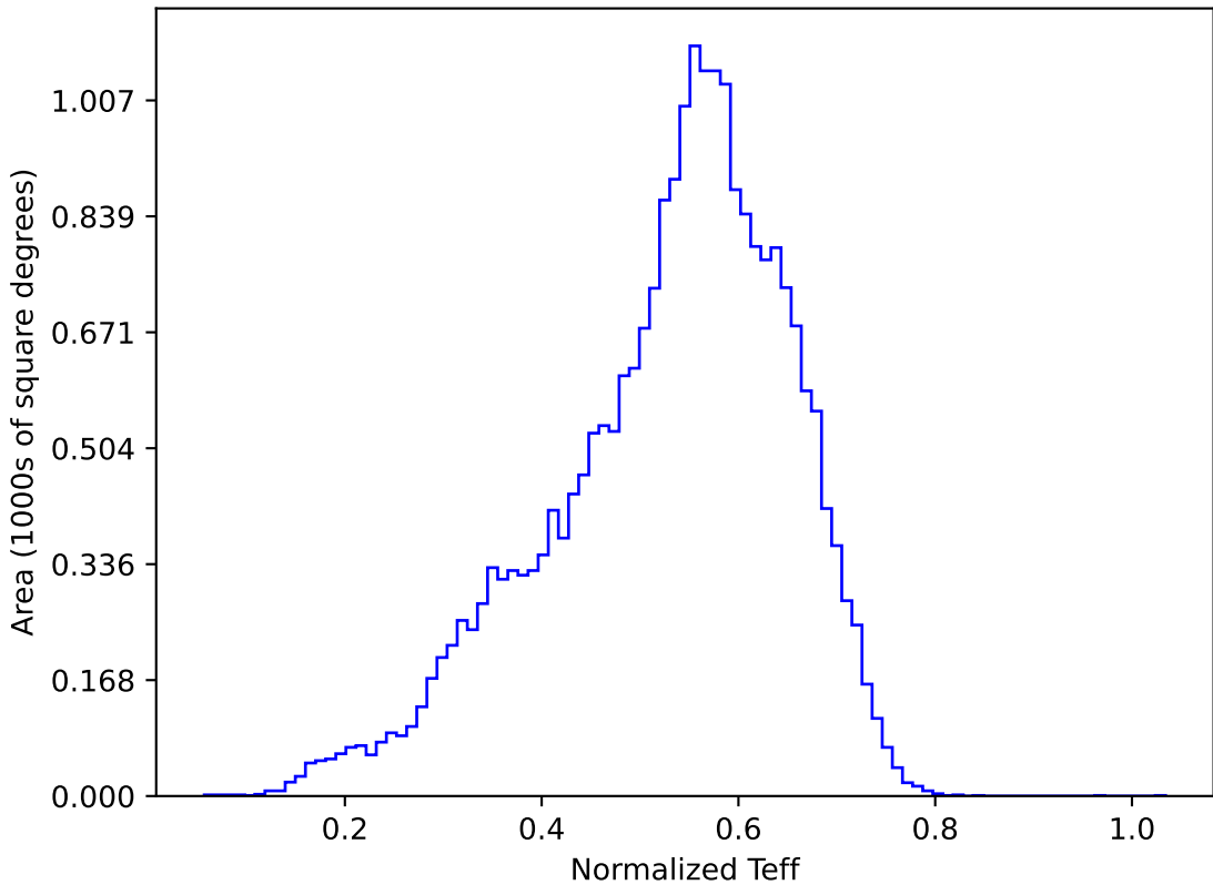
too_elab_r32_d2_ugrizy_v3.4_10yrs All sky y band: Normalized Teff
