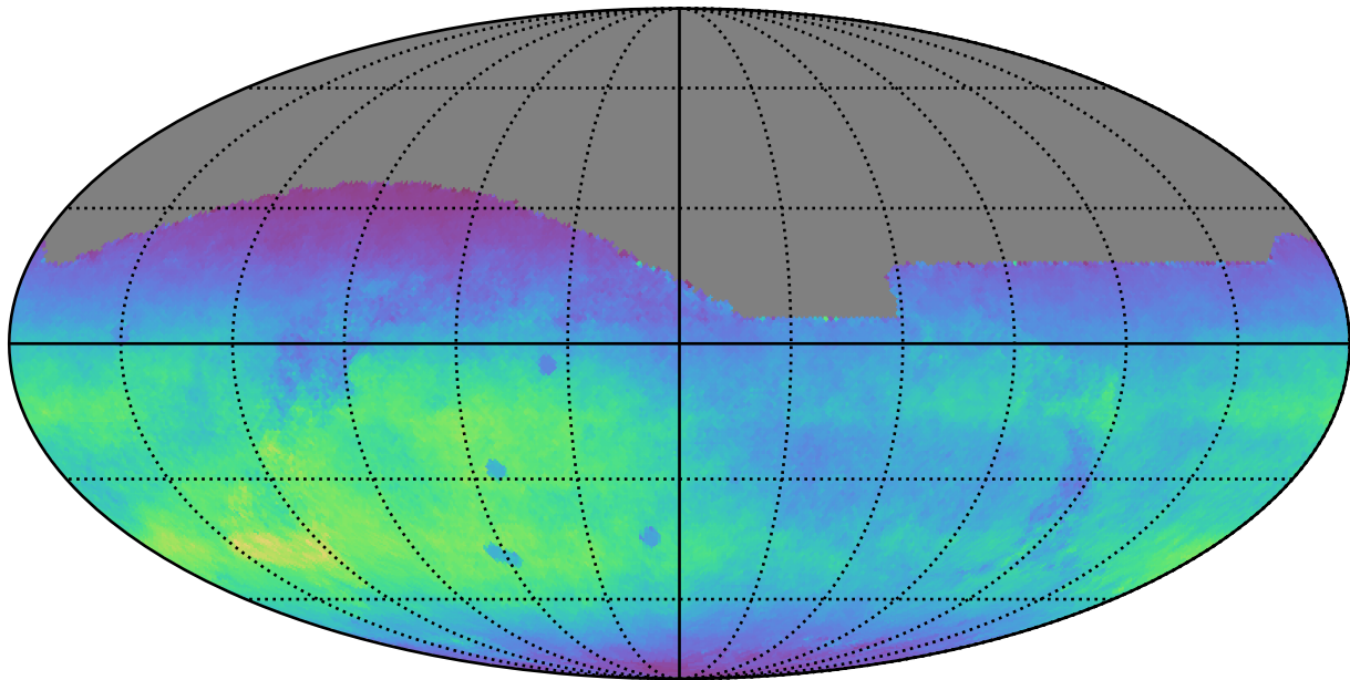
too_elab_r32_d2_ugrizy_v3.4_10yrs All sky r band: Normalized Teff
