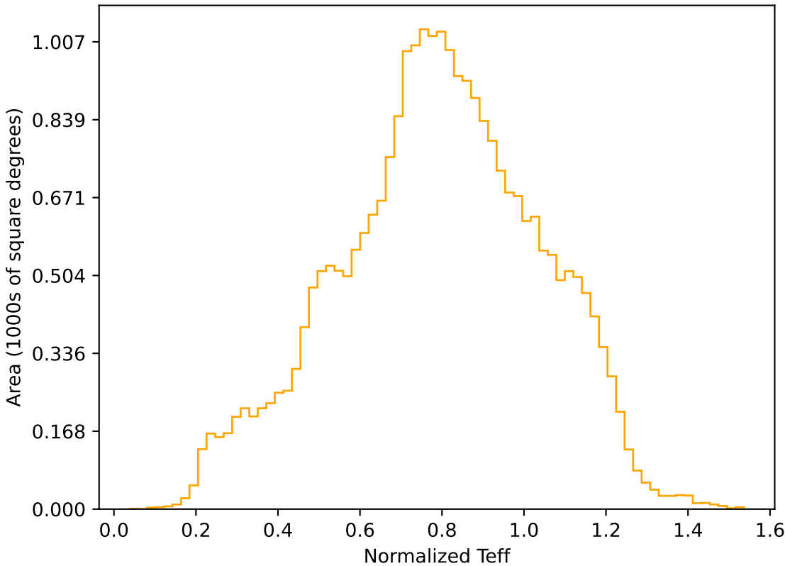
too_elab_r32_d2_ugrizy_v3.4_10yrs All sky r band: Normalized Teff
