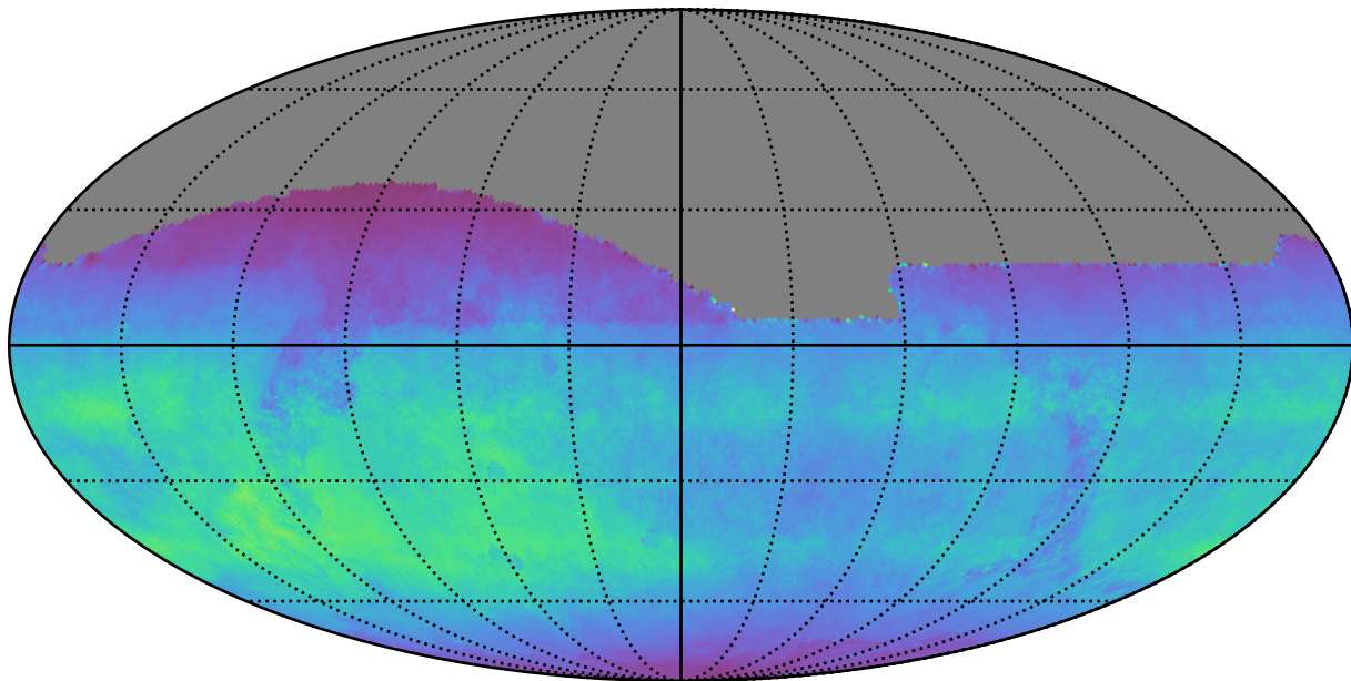
too_elab_r32_d2_ugrizy_v3.4_10yrs All sky i band: Normalized Teff
