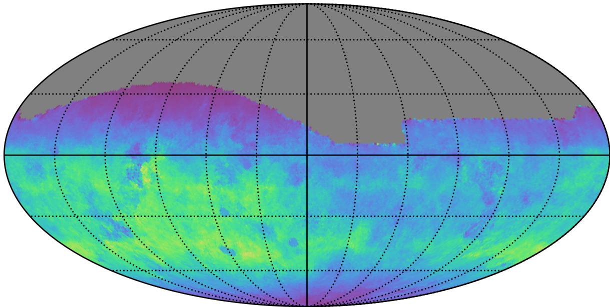
too_elab_r32_d2_ugrizy_v3.4_10yrs All sky g band: Normalized Teff
