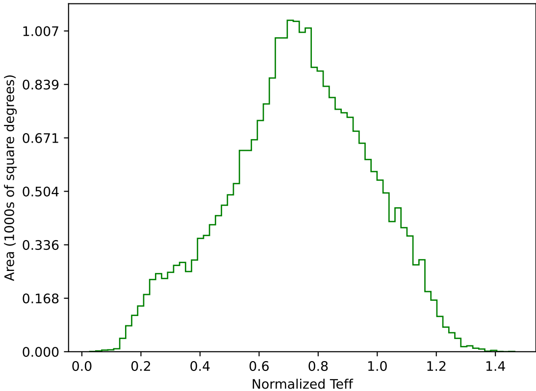
too_elab_r32_d2_ugrizy_v3.4_10yrs All sky g band: Normalized Teff
