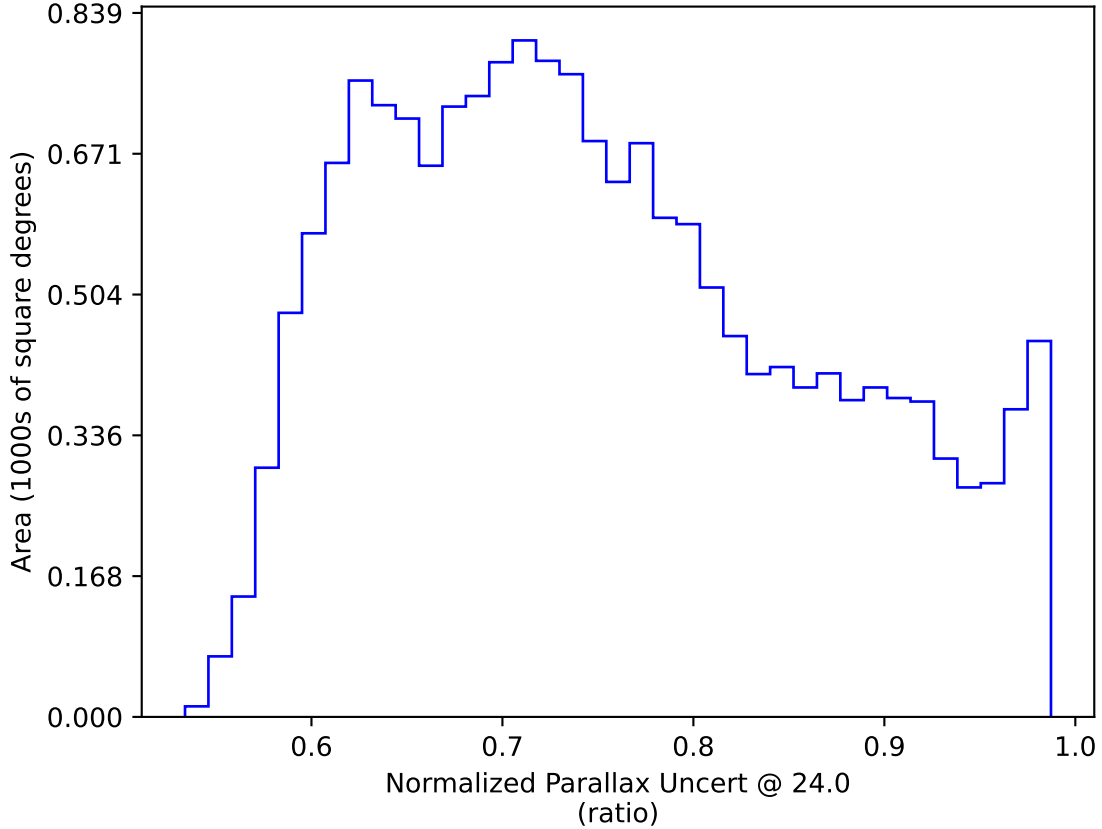
too_elab_r32_d2_ugrizy_v3.4_10yrs WFD: Normalized Parallax Uncert @ 24.0
