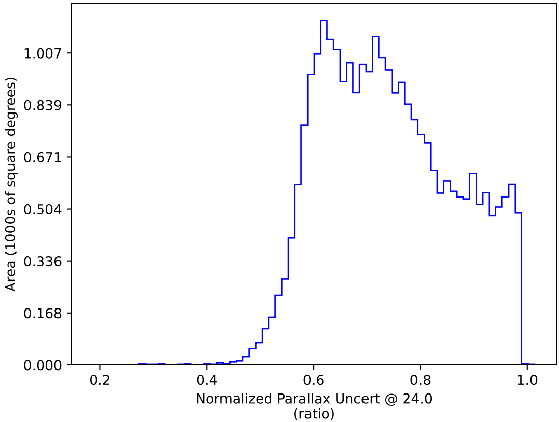
too_elab_r32_d2_ugrizy_v3.4_10yrs All sky: Normalized Parallax Uncert @ 24.0
