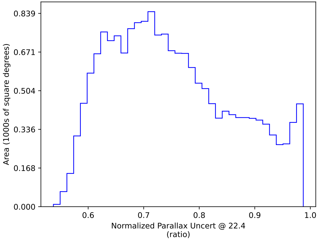
too_elab_r32_d2_ugrizy_v3.4_10yrs WFD: Normalized Parallax Uncert @ 22.4
