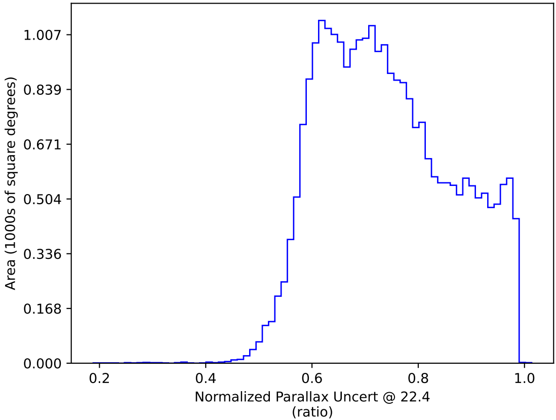
too_elab_r32_d2_ugrizy_v3.4_10yrs All sky: Normalized Parallax Uncert @ 22.4
