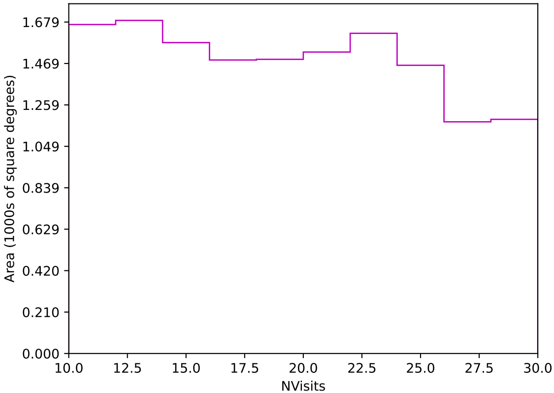
too_elab_r32_d2_ugrizy_v3.4_10yrs Yr 3-4 z band: NVisits
