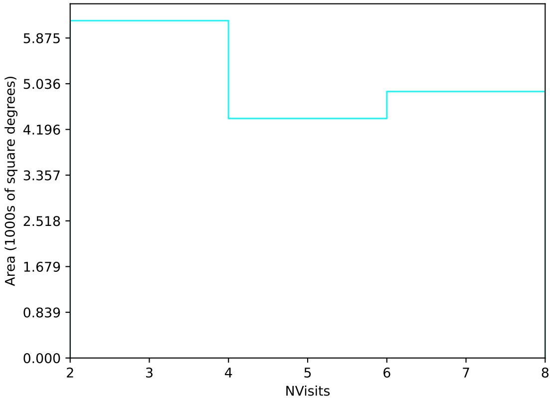
too_elab_r32_d2_ugrizy_v3.4_10yrs Yr 3-4 u band: NVisits
