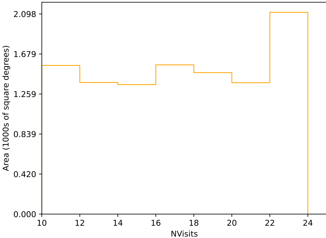
too_elab_r32_d2_ugrizy_v3.4_10yrs Yr 3-4 r band: NVisits
