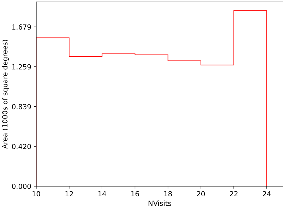
too_elab_r32_d2_ugrizy_v3.4_10yrs Yr 3-4 i band: NVisits
