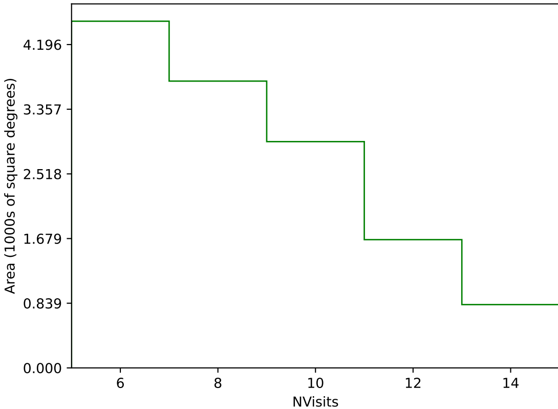
too_elab_r32_d2_ugrizy_v3.4_10yrs Yr 3-4 g band: NVisits
