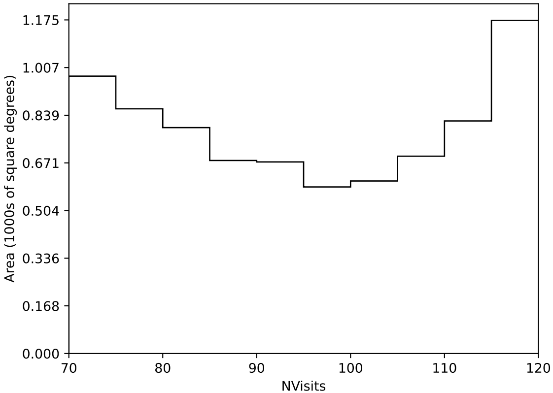
too_elab_r32_d2_ugrizy_v3.4_10yrs Yr 3-4 all bands: NVisits
