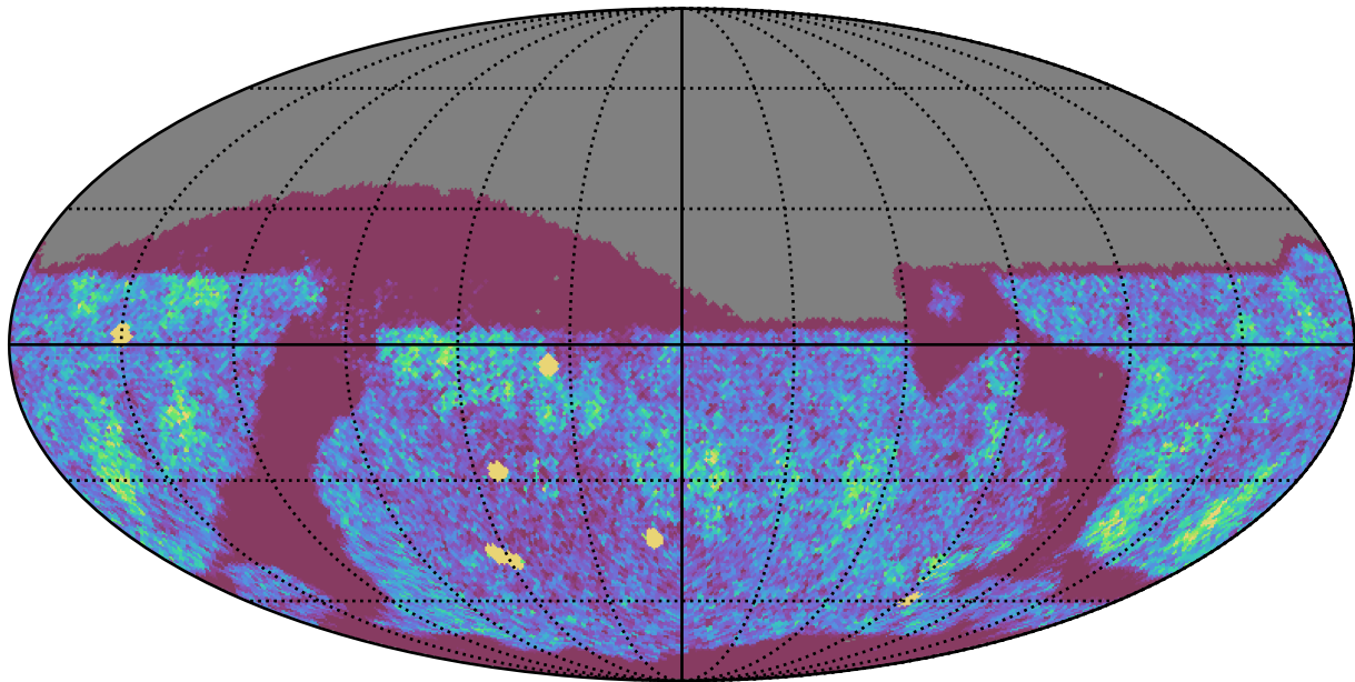
too_elab_r32_d2_ugrizy_v3.4_10yrs Yr 1 z band: NVisits
