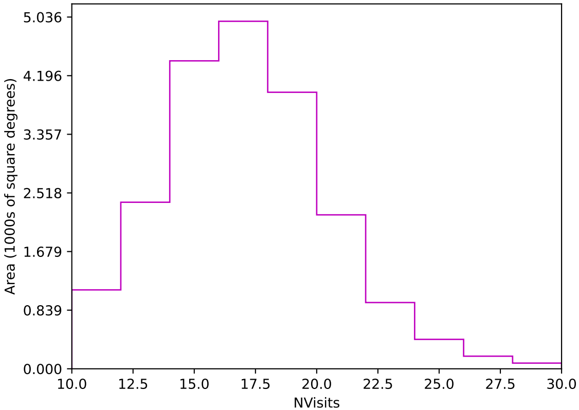
too_elab_r32_d2_ugrizy_v3.4_10yrs Yr 1 z band: NVisits
