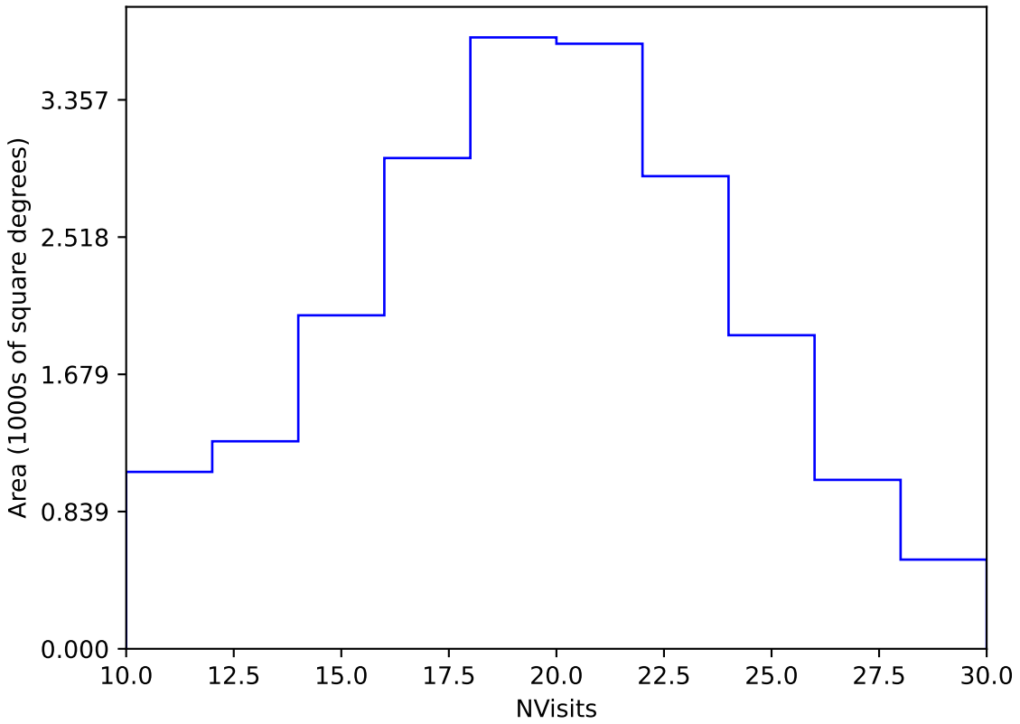
too_elab_r32_d2_ugrizy_v3.4_10yrs Yr 1 y band: NVisits
