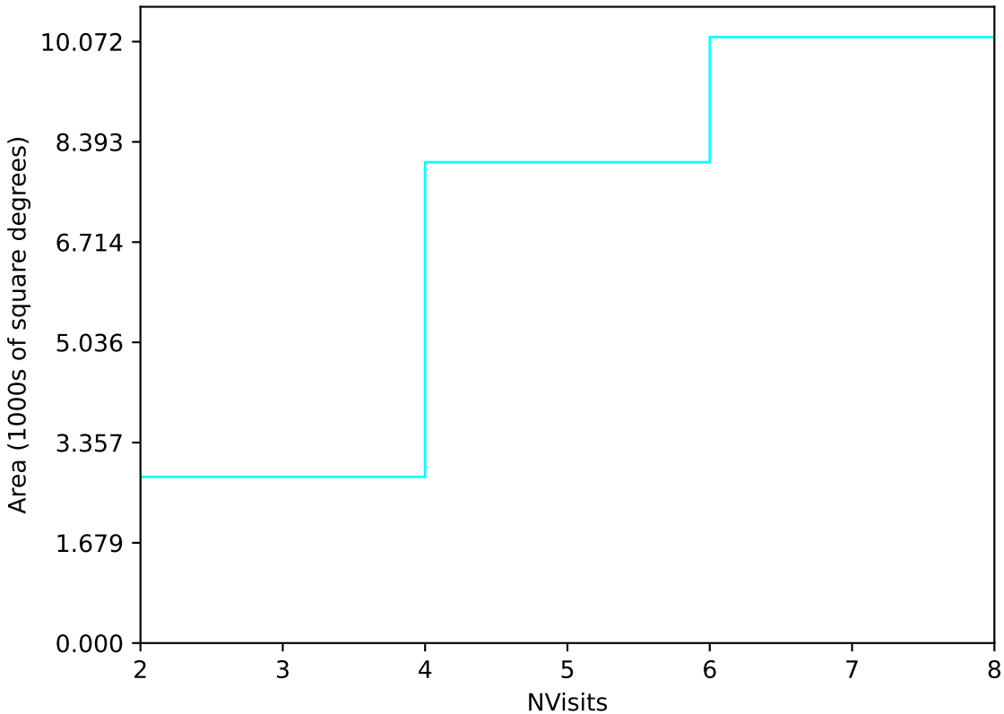
too_elab_r32_d2_ugrizy_v3.4_10yrs Yr 1 u band: NVisits
