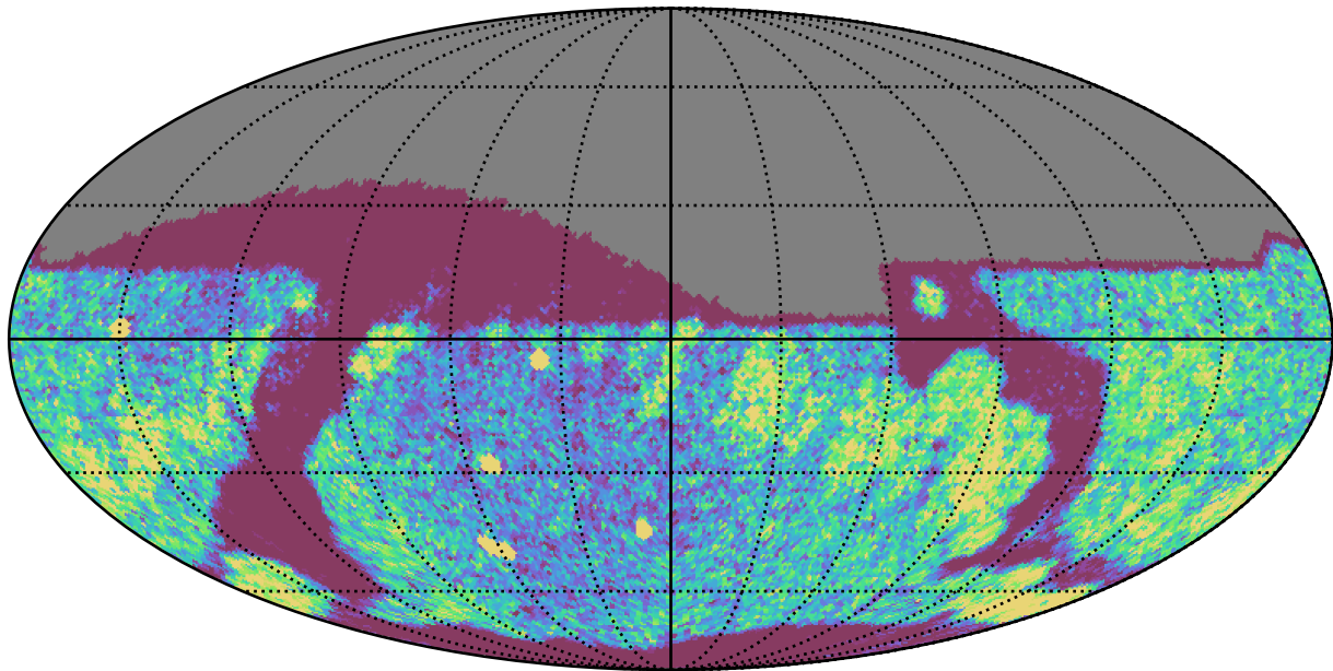
too_elab_r32_d2_ugrizy_v3.4_10yrs Yr 1 r band: NVisits
